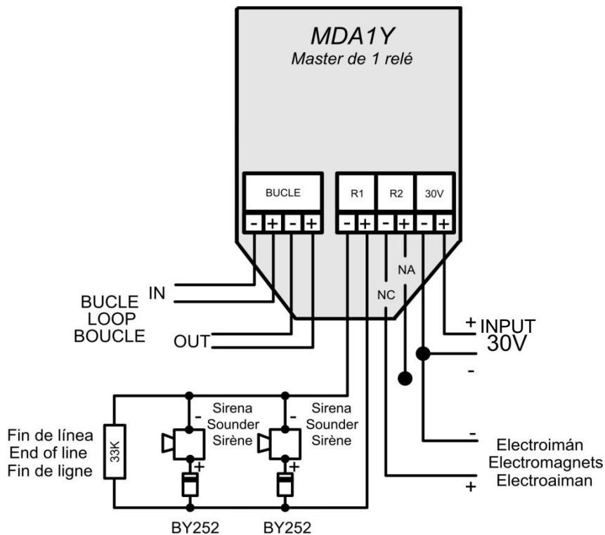
Figure 6. Schéma de raccordement
