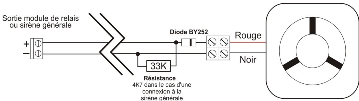
Figure 26. Schéma de raccordement SIR24P
