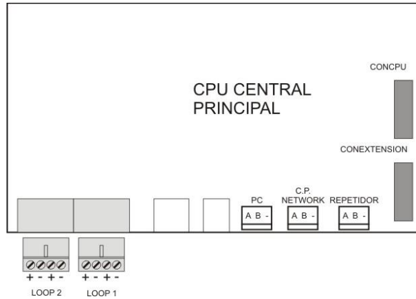
Figure 21. Driver de boucle
