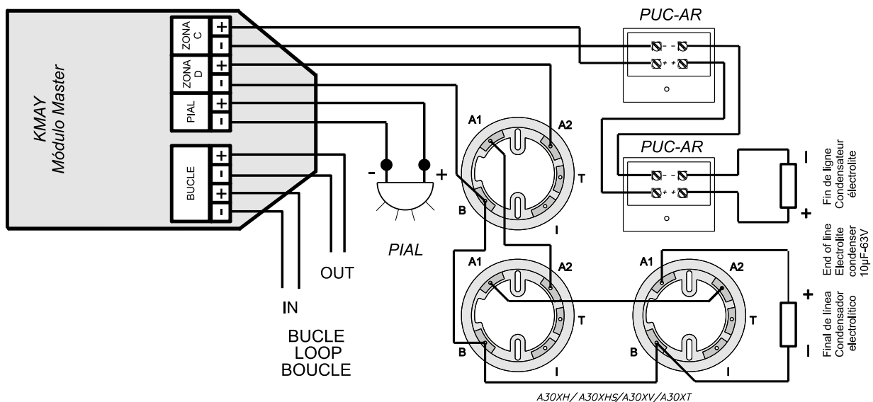
Figure 3. Schéma de raccordement KMAY
