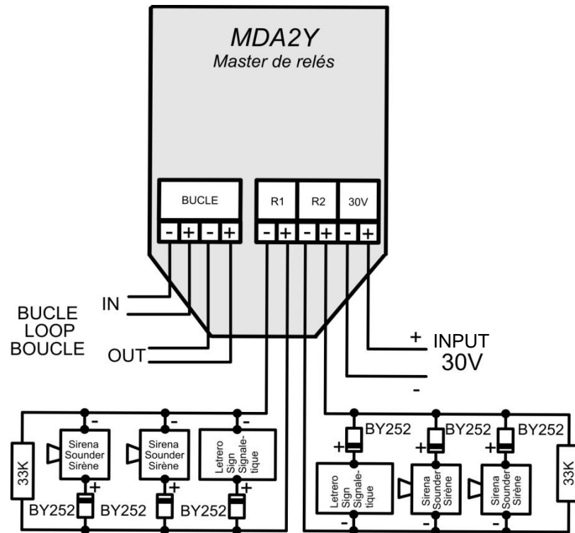
Figure 6. Schéma de raccordement
