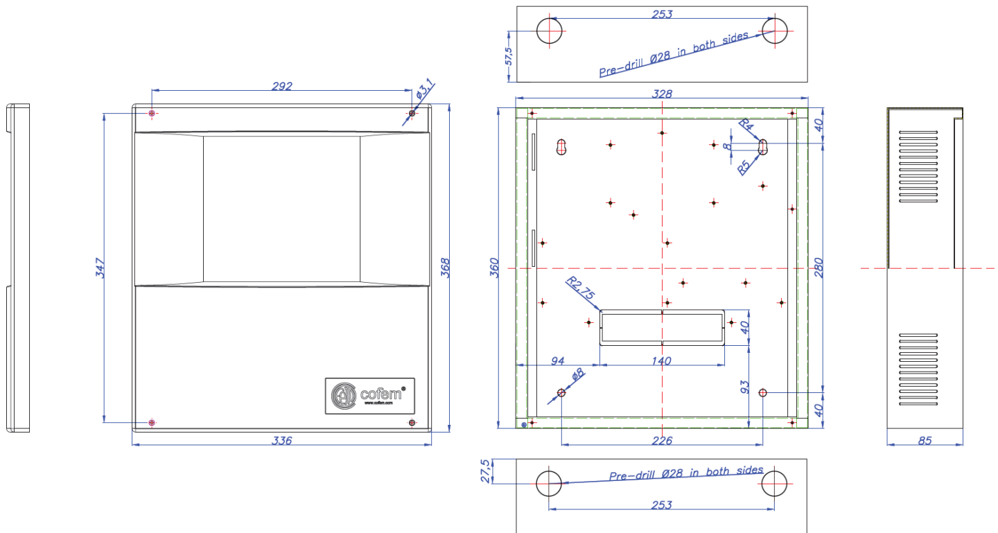
Figure 12. Coffret centrale Compact Lyon
