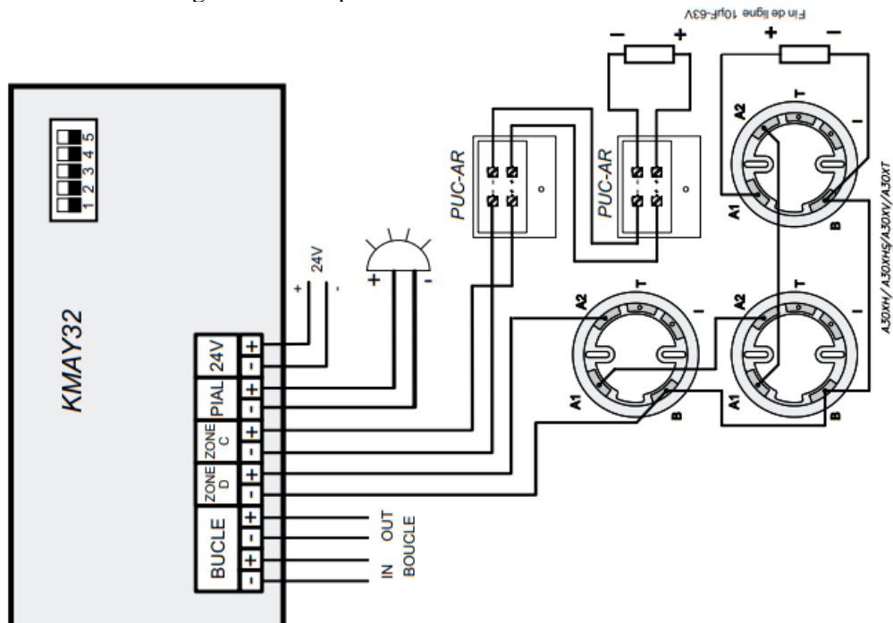
Figure 9. Schéma de raccordement KMAY32
