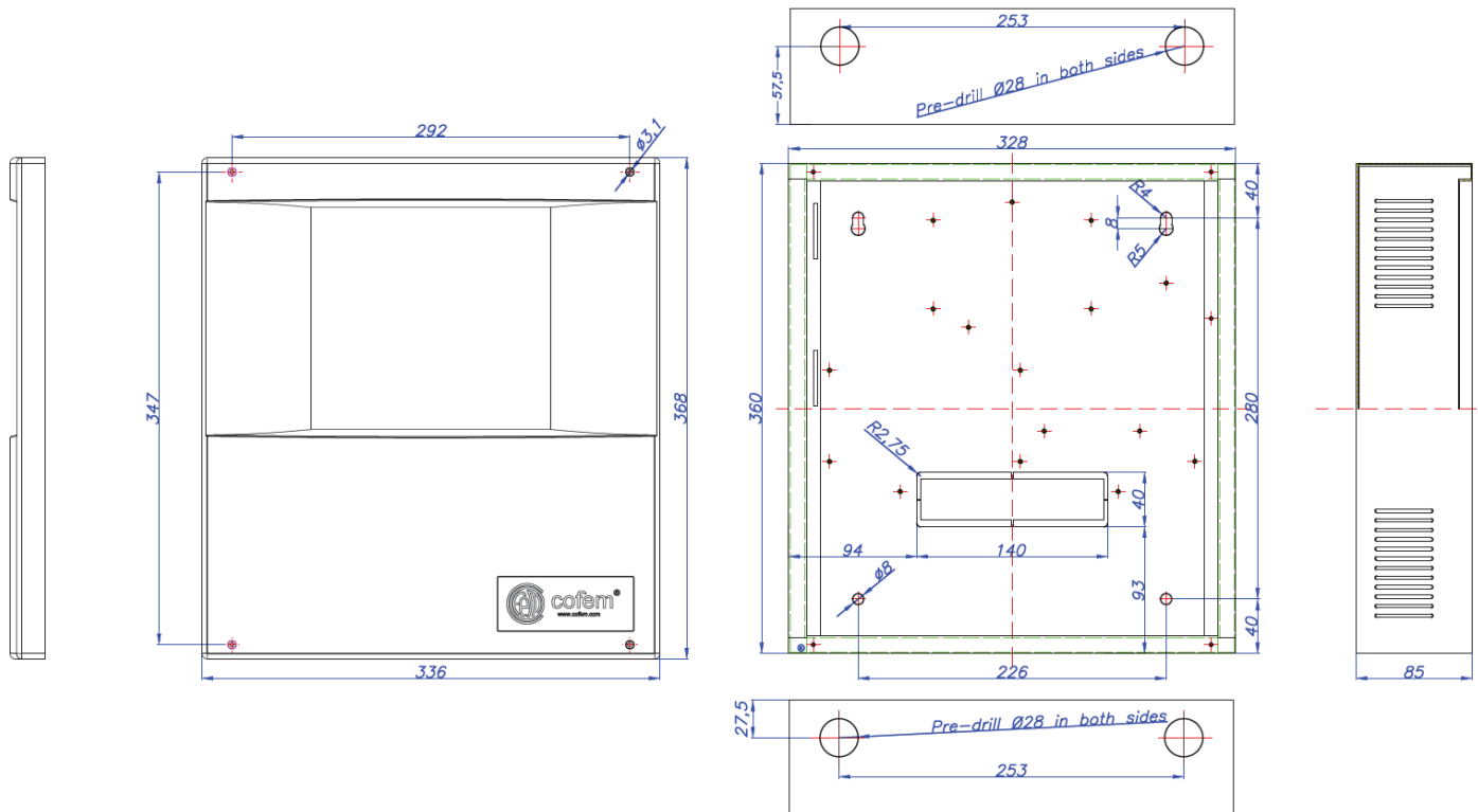
Figure 14. Coffret centrale CLyon
