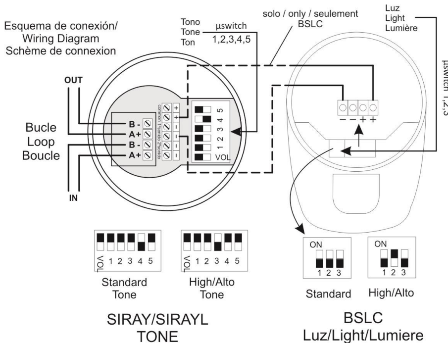
Figure 12. Schéma de raccordement SIRAY / SIRAYL / SIRAY+BSLC
