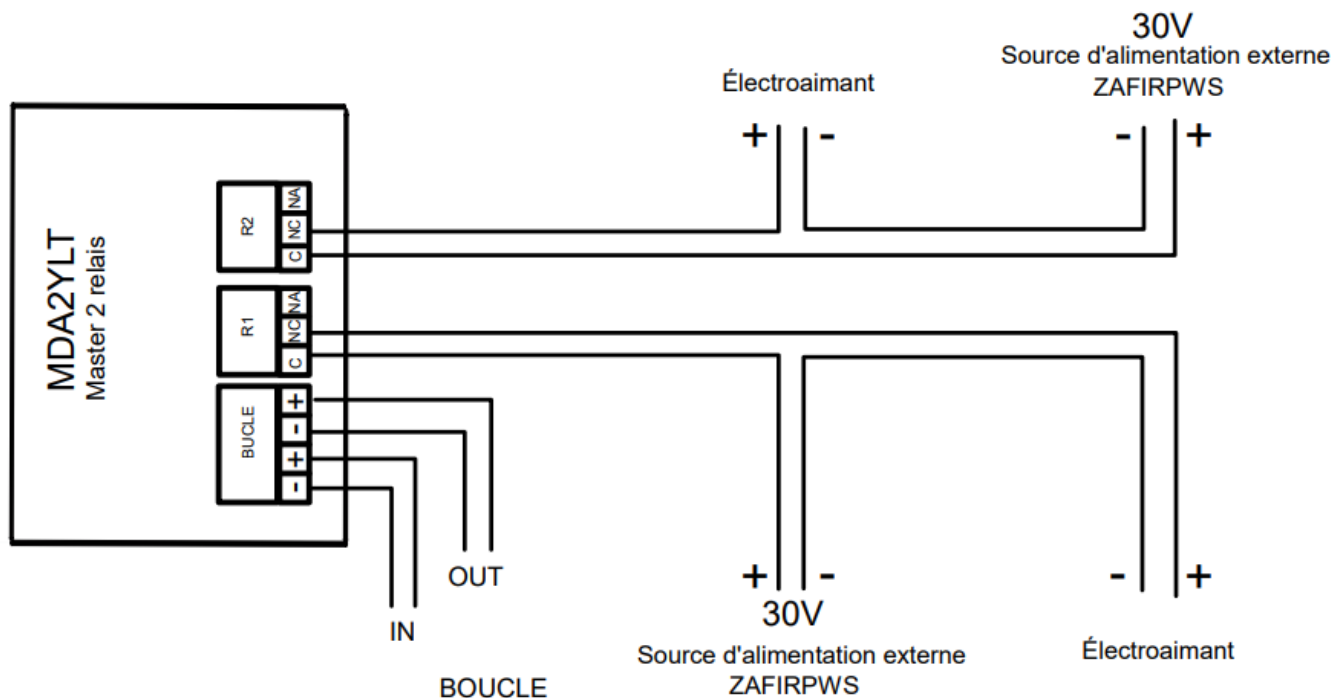
Figure 8. Schéma de raccordement MDA2YLT
