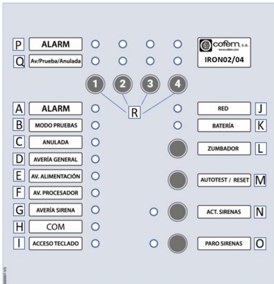
Figura 1: Panel de control de la central IRON02/04
