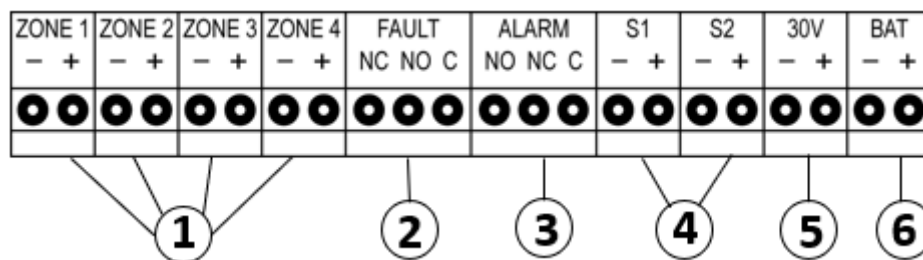
Figure 5: Terminal schema IRON02/04
