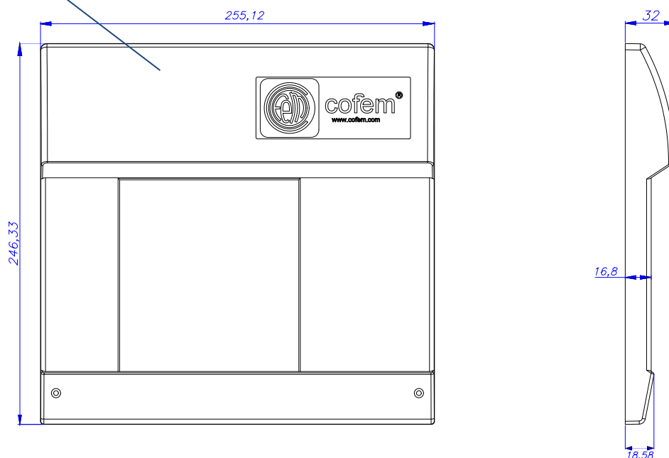
Figure 2: Diagram of box and main door
