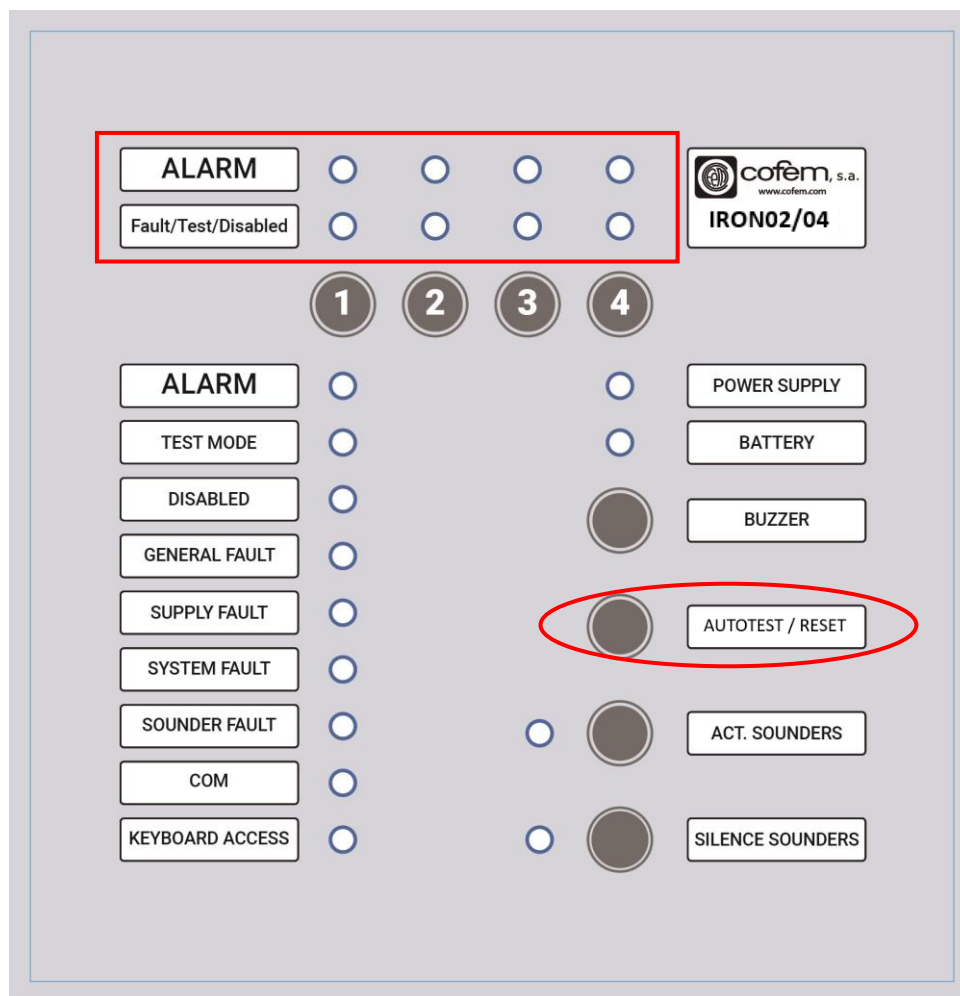
Figure 13: Keys and LEDs for firmware version.
