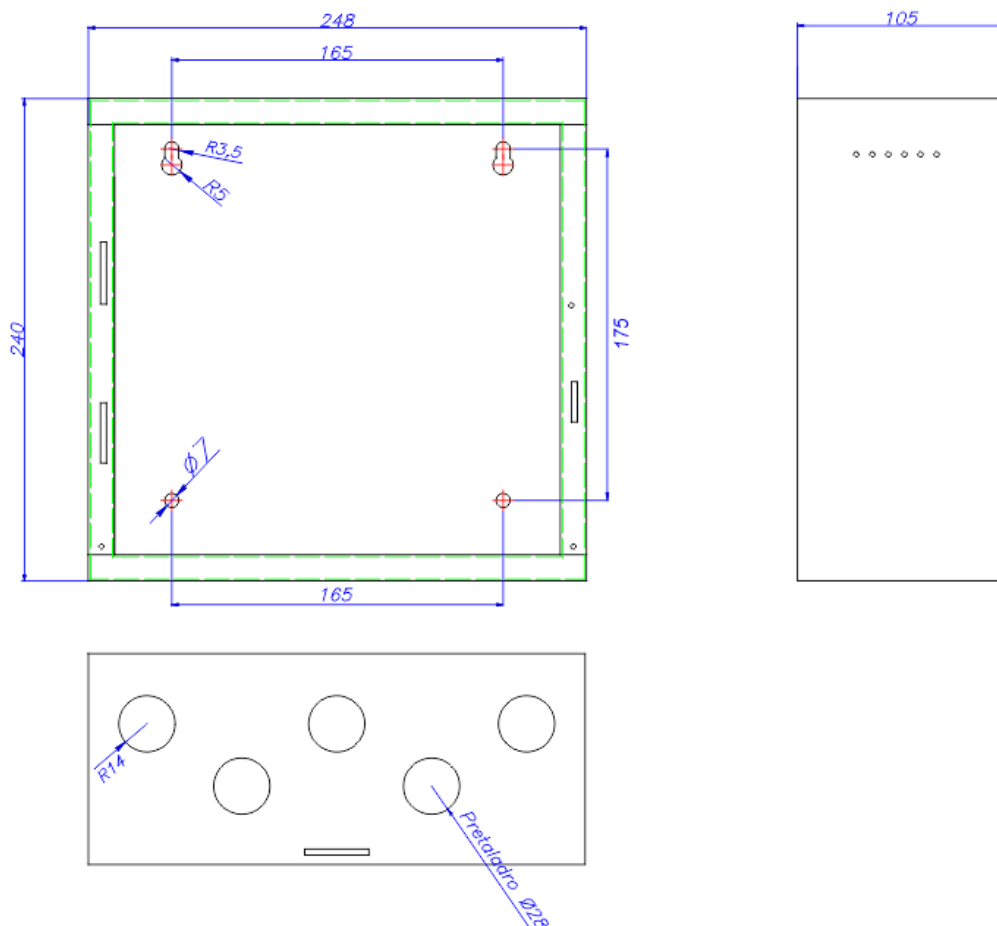
Figure 3: Door and main box measurements (mm).
