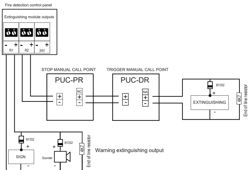
Wiring diagram
