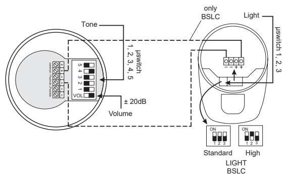
SOUNDER SIR24B + BSLC
