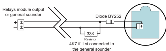
Wiring diagram CA6
