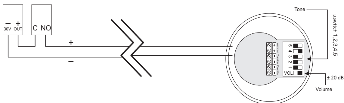
Wiring diagram
