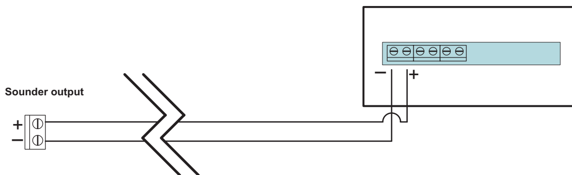
Wiring diagram
