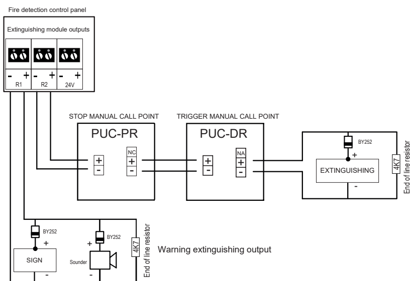
Wiring diagram
