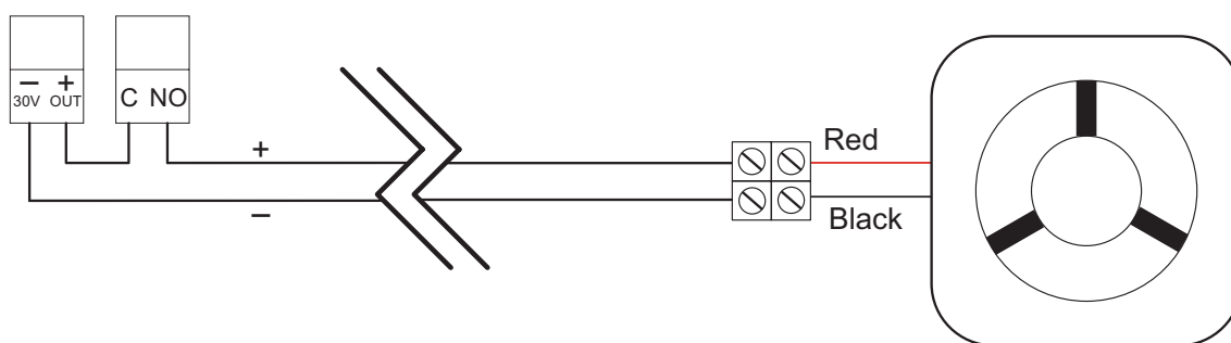
Wiring diagram
