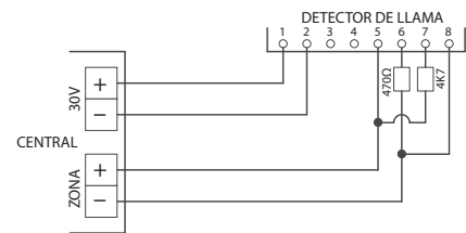
Wiring diagram
