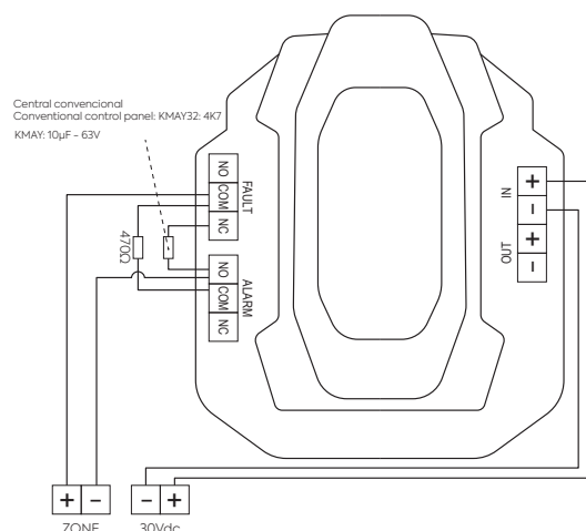
DLRC connection diagram
