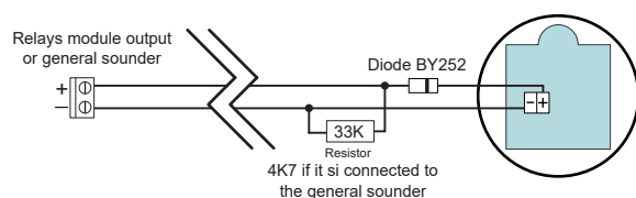
Wiring diagram CA6
