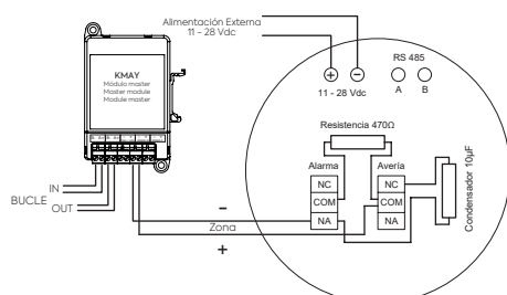
DLRCM60 / DLRCM120 connection diagram
